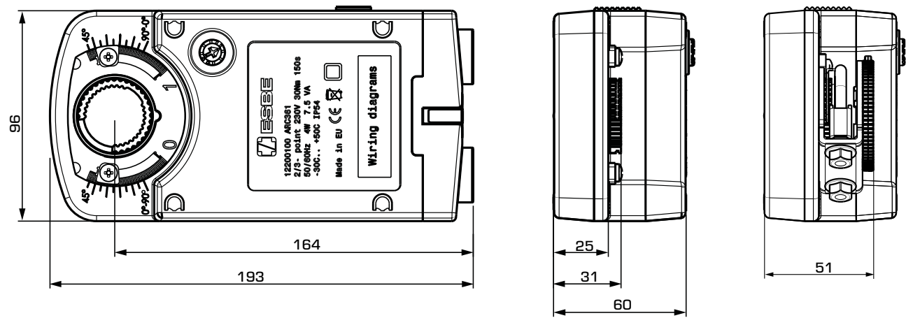
Actuator Series ARC300
